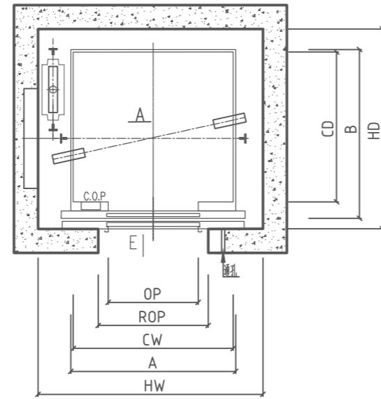
Hoistway Plan
