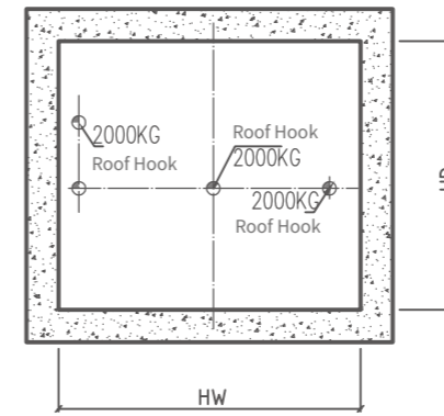
Shaft Hook Plan
