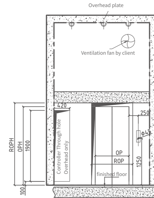
TOP Floor Front View
